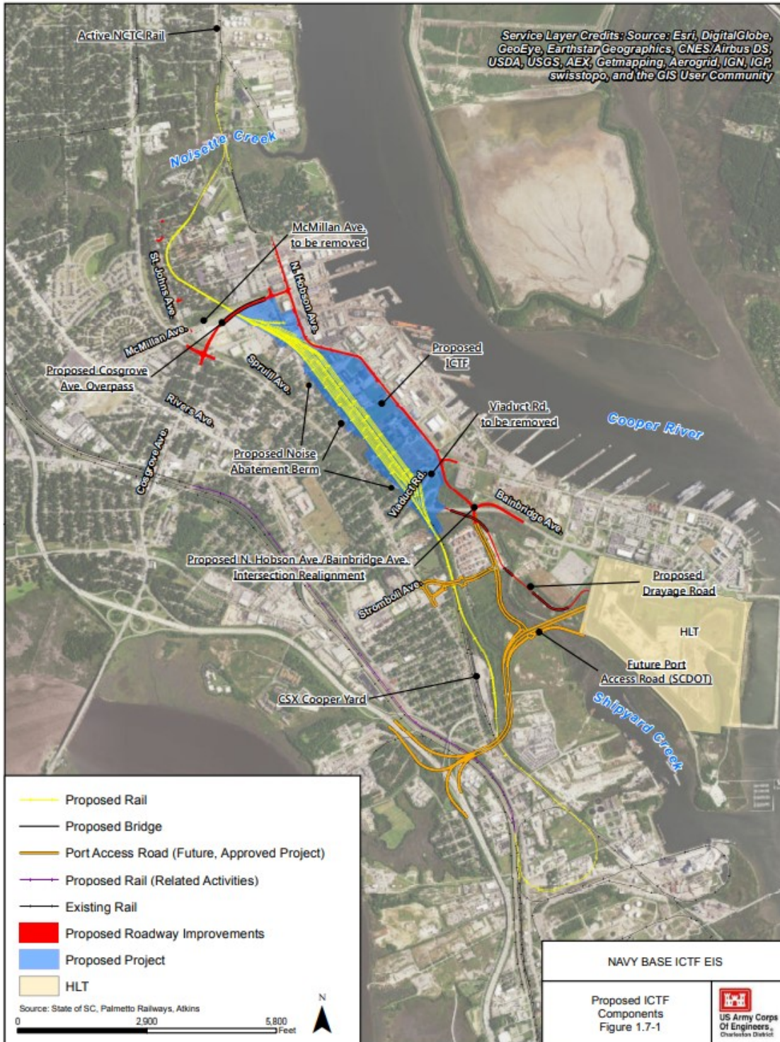
Navy Base Intermodal Container Transfer Facility (ICTF) Components (Source: State of SC, Palmetto Railways), 2018
